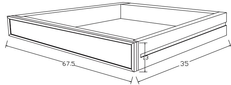
DRAWER
