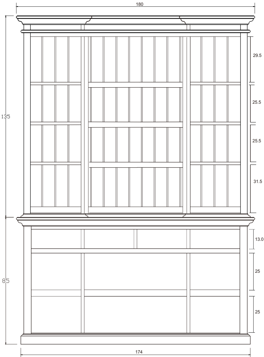
FRONT OPEN
