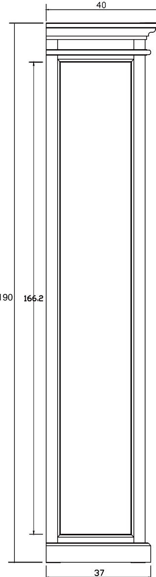
SIDE VIEW
