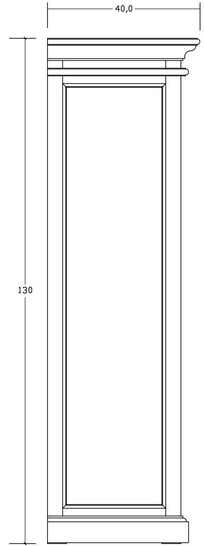
SIDE VIEW
